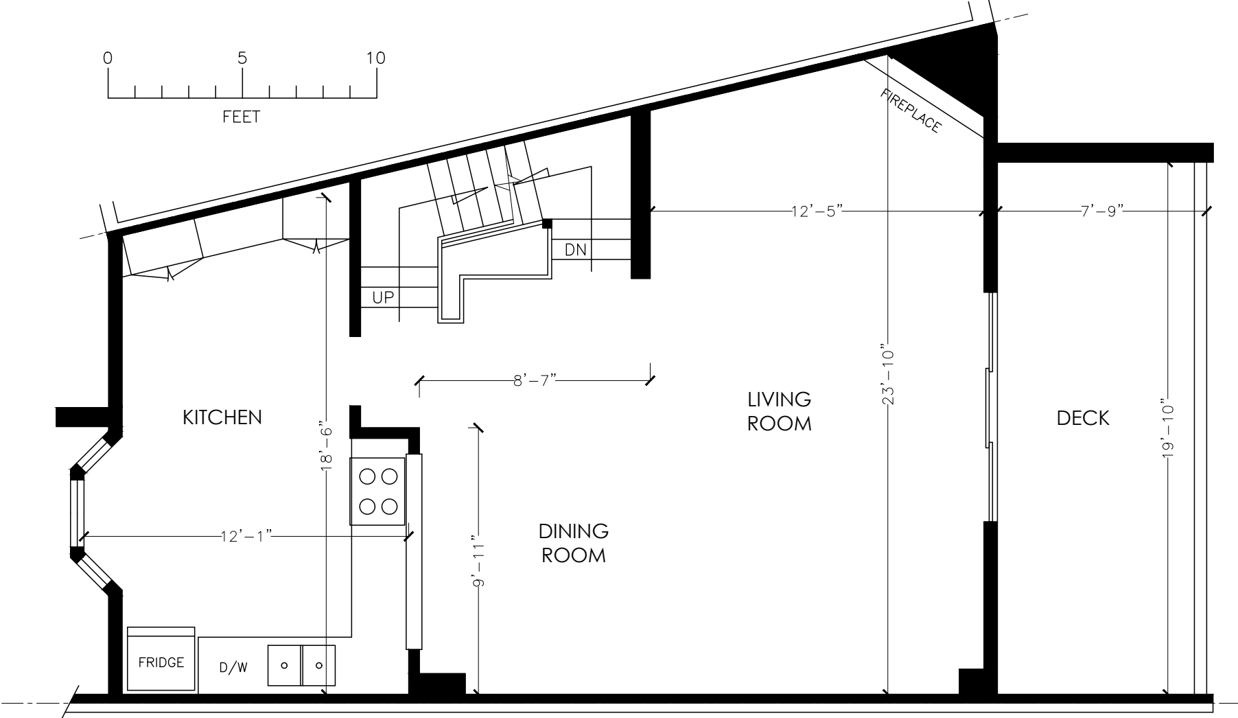
SECOND FLOOR FLOOR AREA 716 SQUARE FEET
