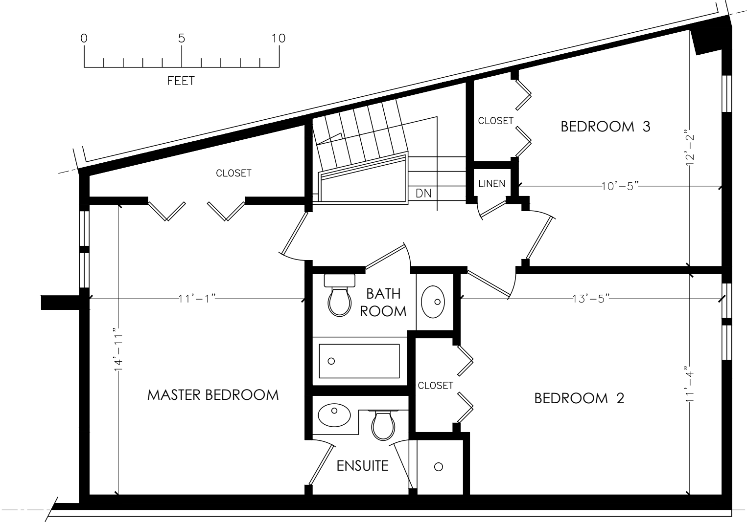
THIRD FLOOR FLOOR AREA 719 SQUARE FEET
