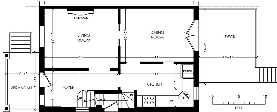
MAIN FLOOR FLOOR AREA 608 SQUARE FEET
