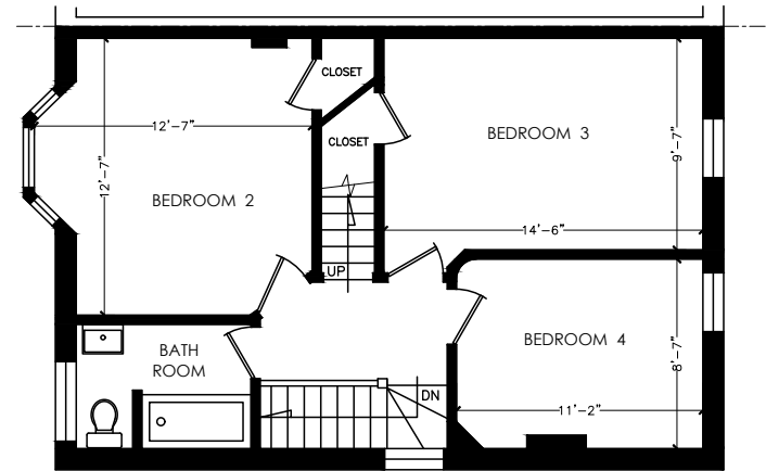
SECOND FLOOR FLOOR AREA 615 SQUARE FEET
