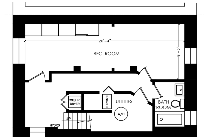
BASEMENT FLOOR AREA 608 SQUARE FEET
