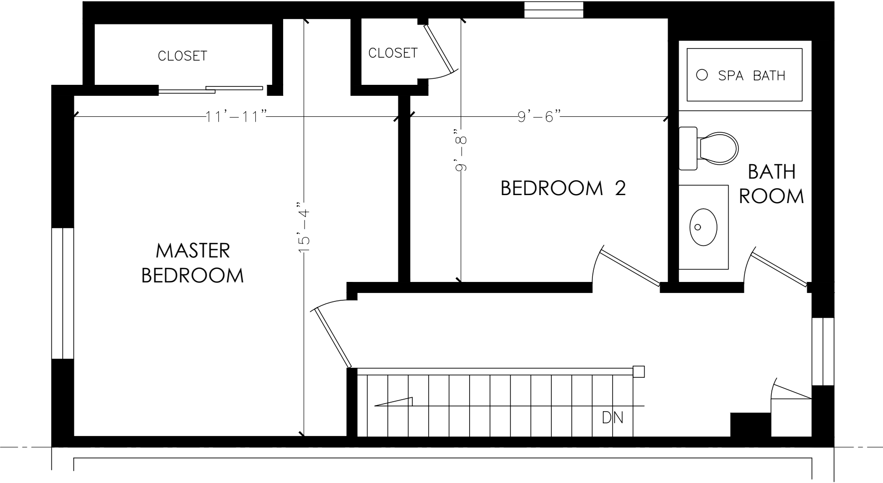
SECOND FLOOR FLOOR AREA 465 SQUARE FEET
