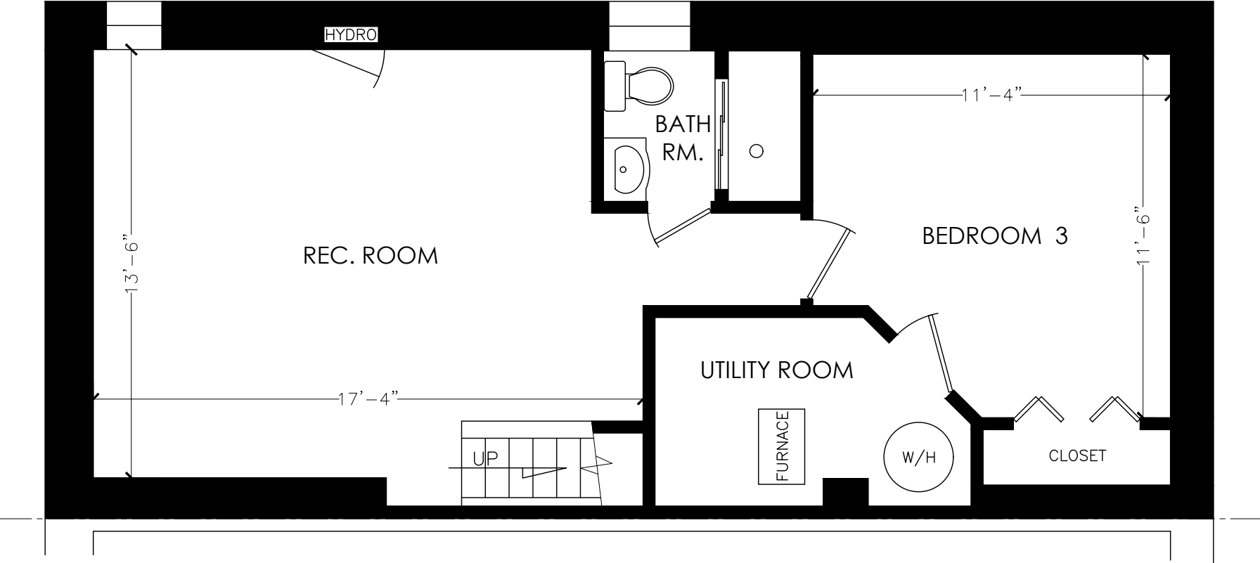
BASEMENT FLOOR AREA 602 SQUARE FEET
