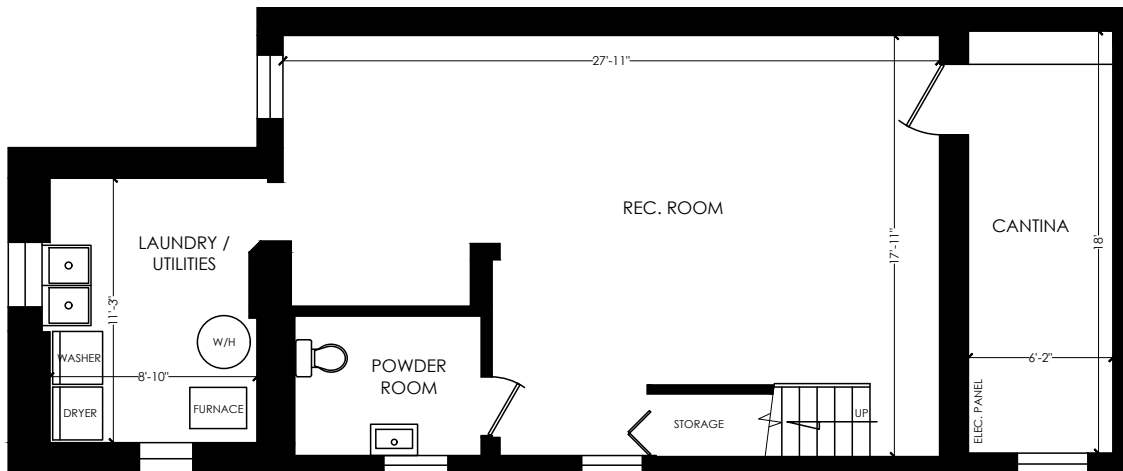
BASEMENT FLOOR AREA 749 SQUARE FEET
