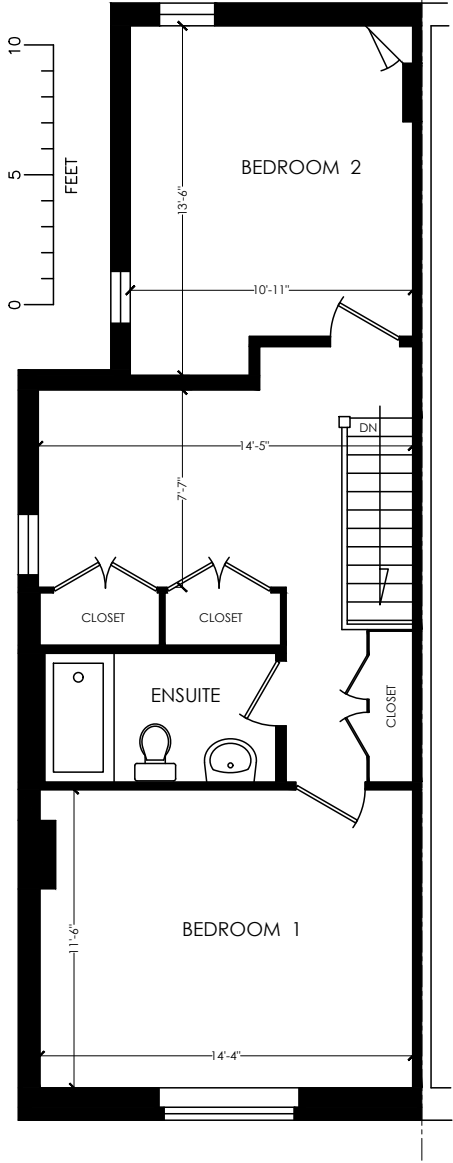
SECOND FLOOR FLOOR AREA 618 SQ. FT.
